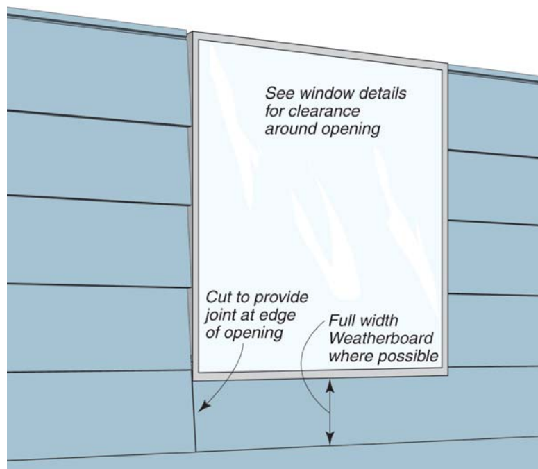
FIG 7: Window Openings
