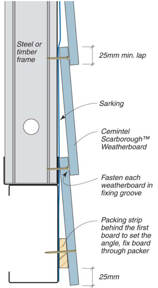
FIG 2: Screw Fixing with Timber Packing Strip
