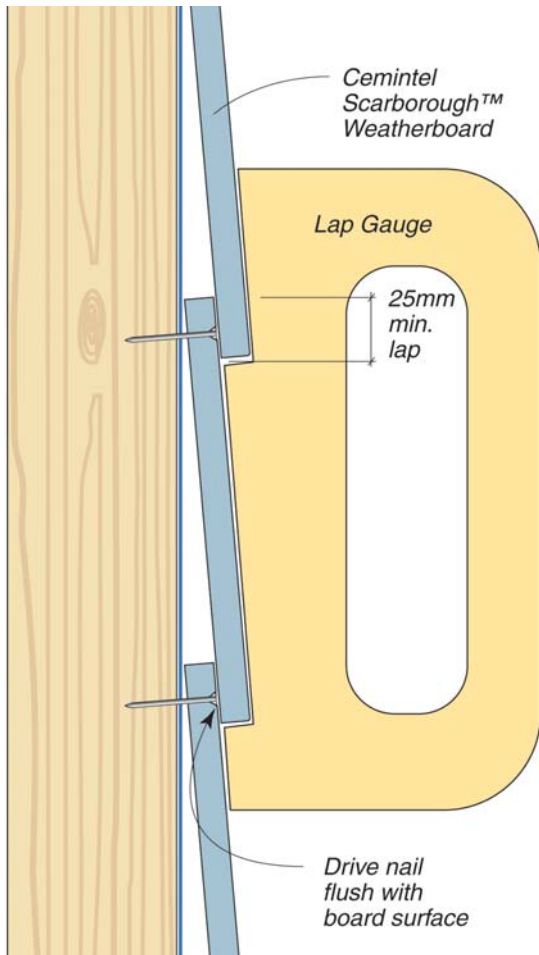
FIG 5: Weatherboard Set-out
