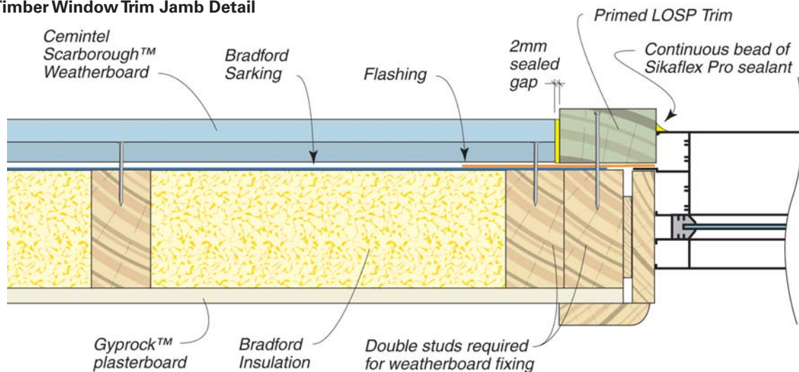
FIG 19: Timber Window Trim Jamb Detail
