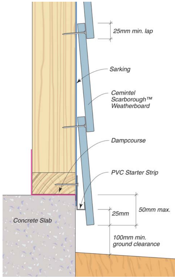
FIG 1: Base Detail with PVC Starter Strip
