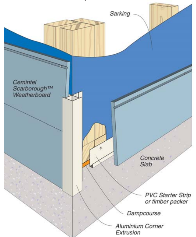
FIG 4: Installation Start-up Detail
