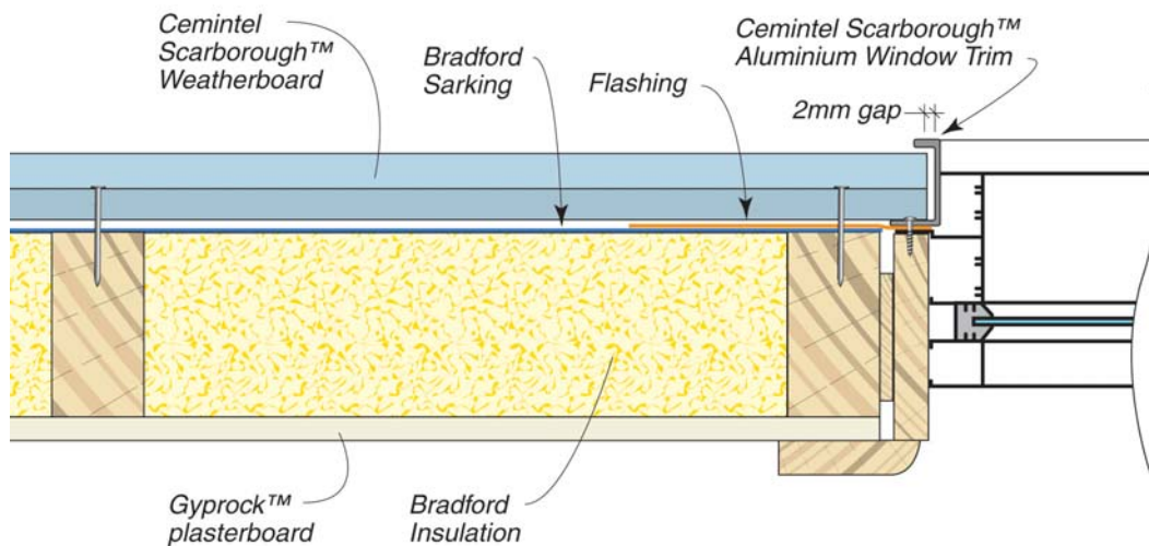
FIG 17: Aluminium Window Trim Jamb Detail
