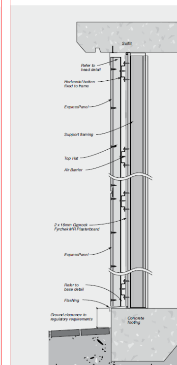
Typical Commercial ExpressPanel External Fire Rated installation. Pressure Equalised Ventilated Cavity System
