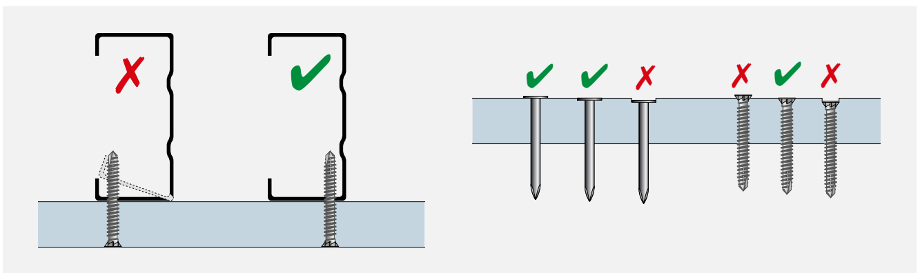
FIGURE 8.16 FASTENER POSITION AND FASTENER DRIVING
