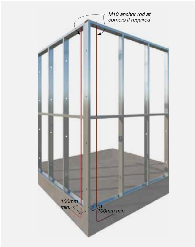
FIGURE 8.15 ANCHOR ROD DETAIL FOR STRUCTURAL BRACING STEEL FRAME
