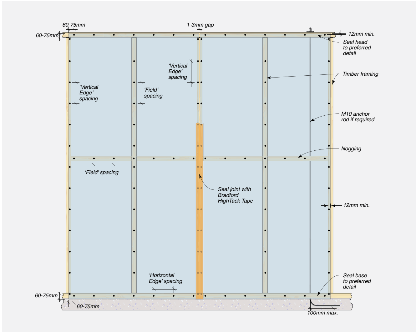
FIGURE 6.05 SHEET FIXING FOR STRUCTURAL BRACING - VERTICAL SHEETING - TIMBER FRAMING
