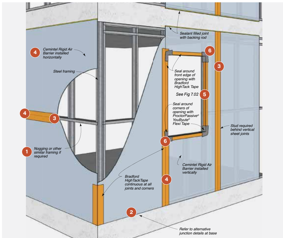
FIGURE 7.01 TYPICAL RIGID AIR BARRIER INSTALLATION
