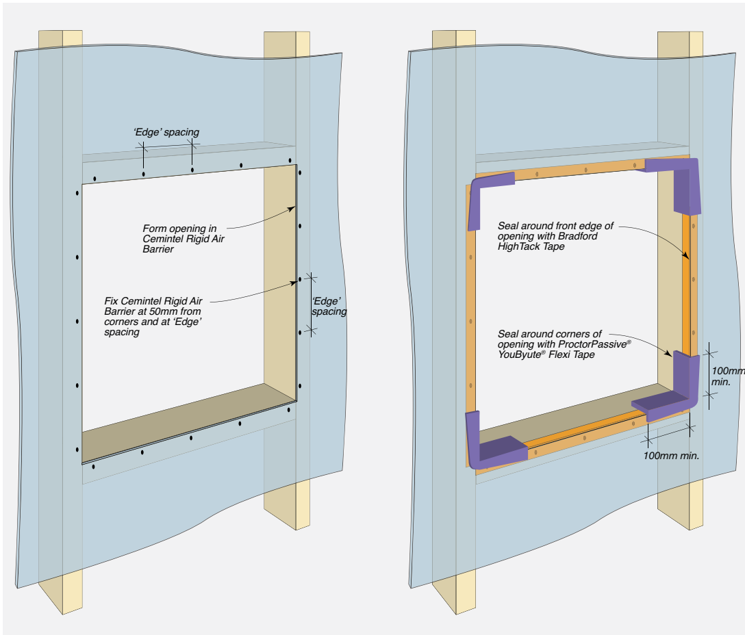
FIGURE 7.02 TREATMENT AT WINDOW/DOOR OPENINGS – RIGID AIR BARRIER
