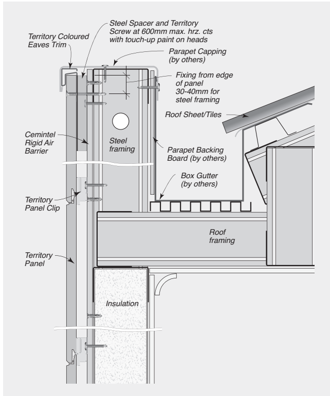
FIGURE 8.67 Parapet Details – Horizontal Steel Framing
