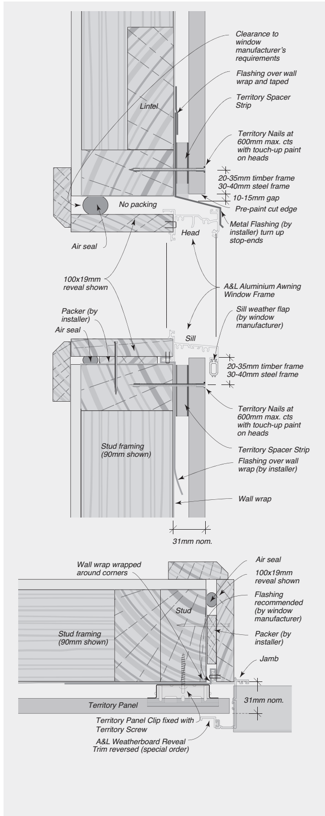
FIGURE 8.22 A&amp;L Aluminium Awning Window with Weatherboard Trim
