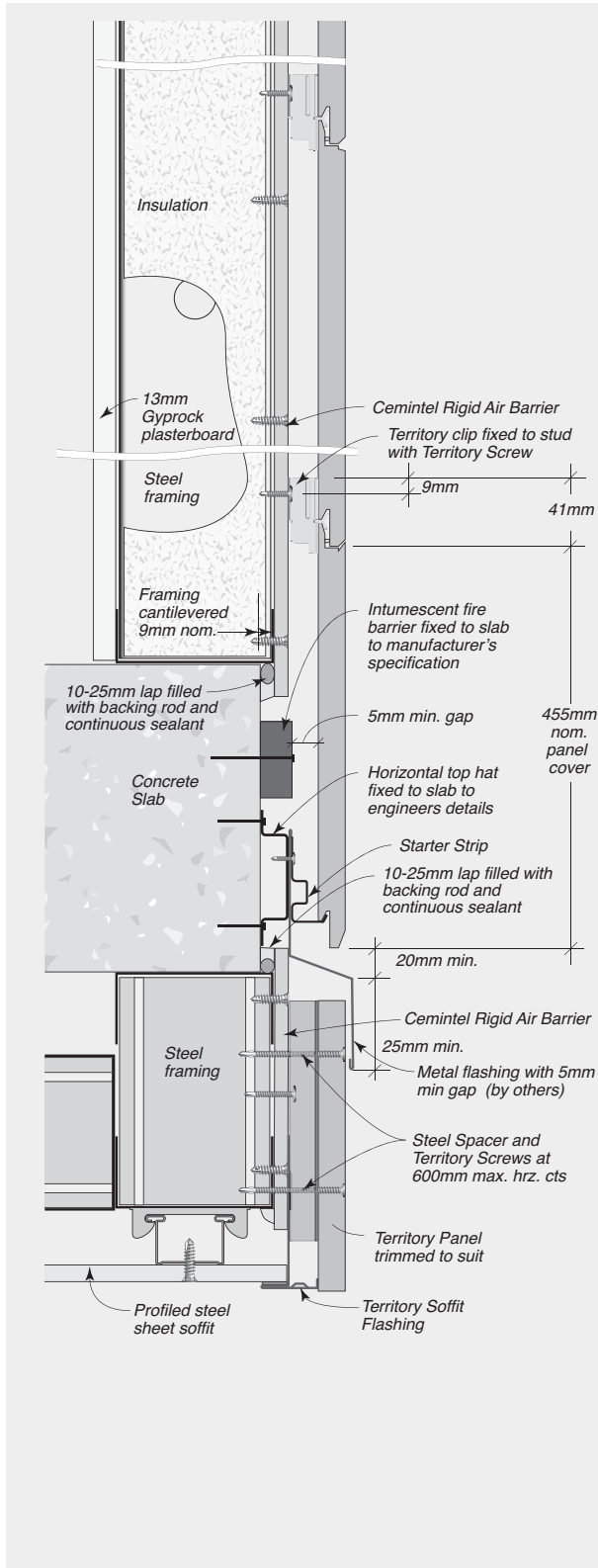
FIGURE 8.63 Interstorey Junction with Metal Ceiling
