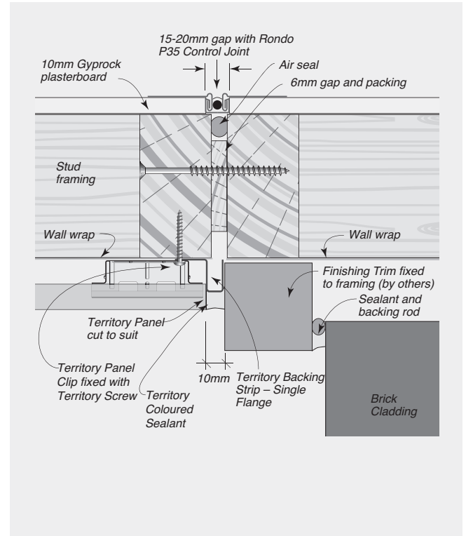
FIGURE 8.18 Junction – Recessed with Brick Veneer
