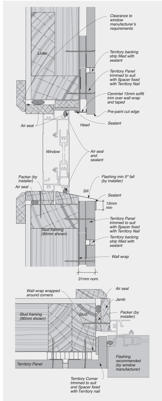
FIGURE 8.29 Window Reveal
