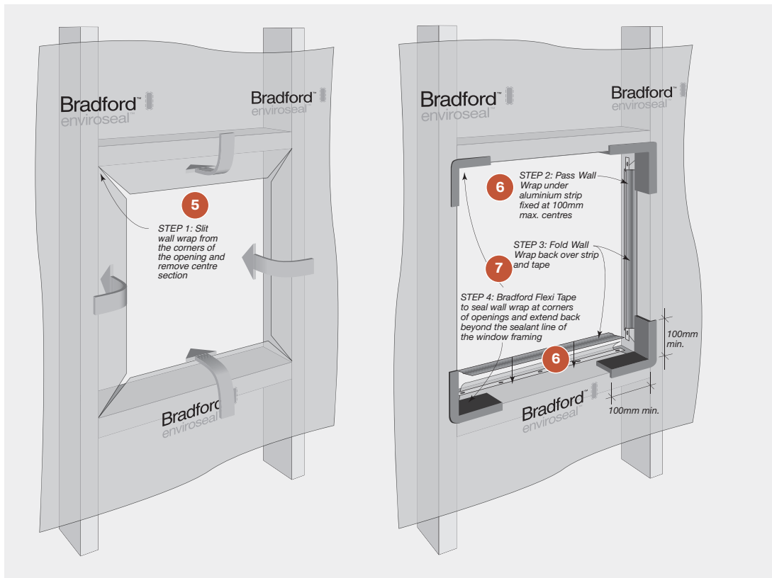
FIGURE 7.04 Treatment at Window/Door Openings - Soft Air Barrier
