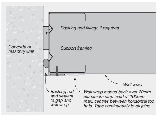
FIGURE 8.73 Abutment to Concrete or Masonry Wall
