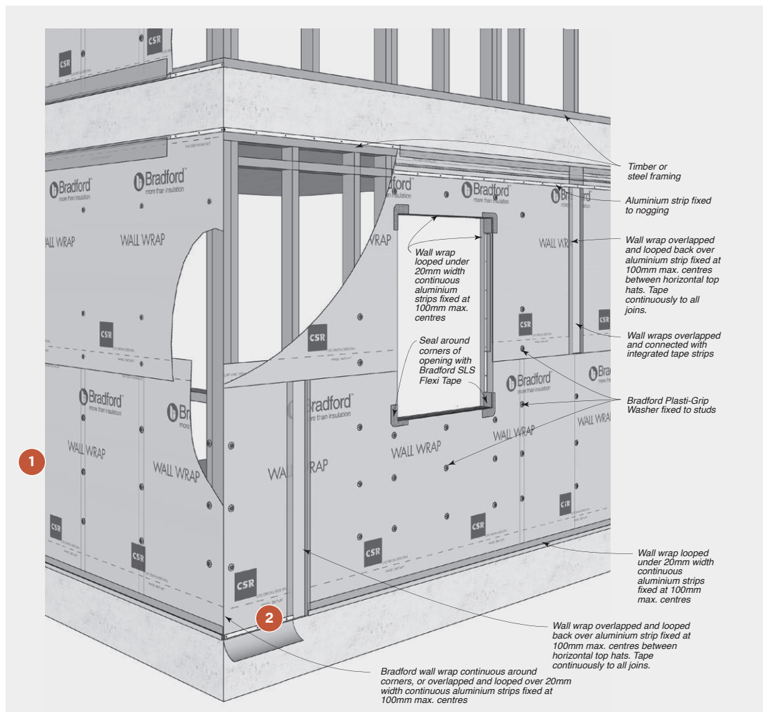
FIGURE 7.03 Typical Soft Air Barrier Installation
