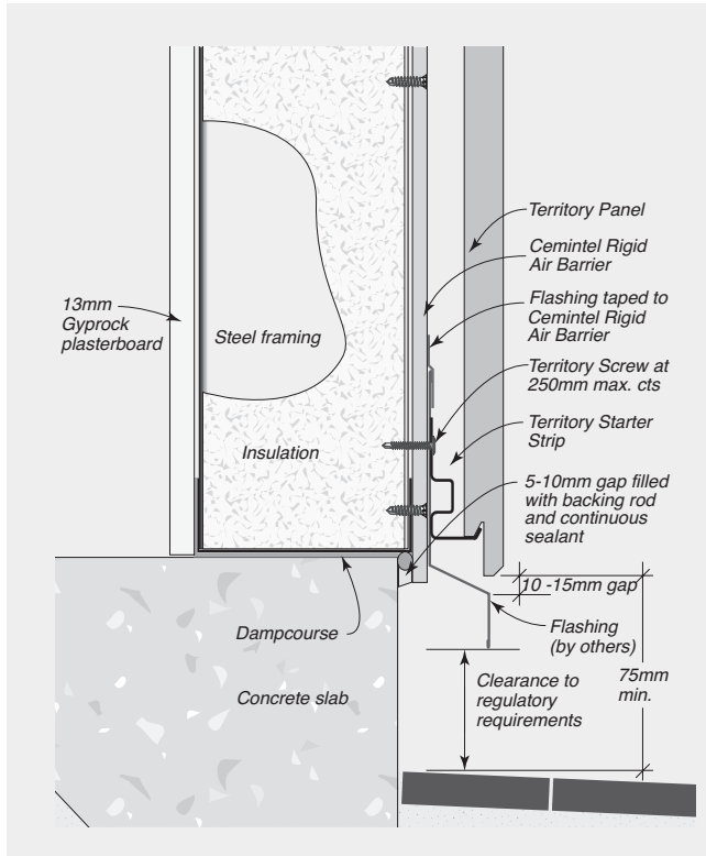
FIGURE 8.53 Base Detail
