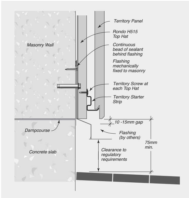
FIGURE 8.42 Typical Base
