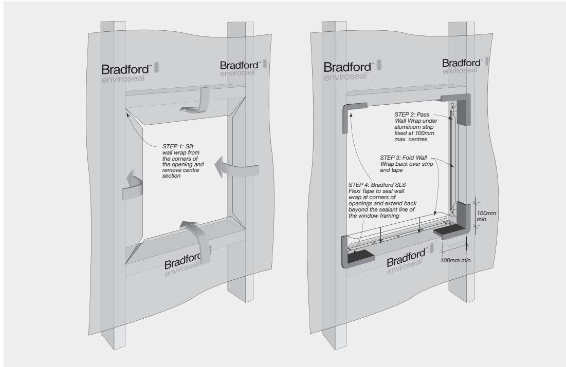
FIGURE 8.82 Wall Wrap Installation at Window/Door Opening
