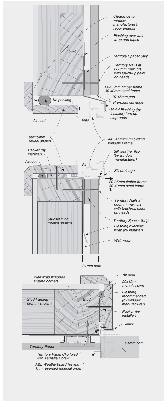
FIGURE 8.23 A&amp;L Aluminium Sliding Window with Weatherboard Trim
