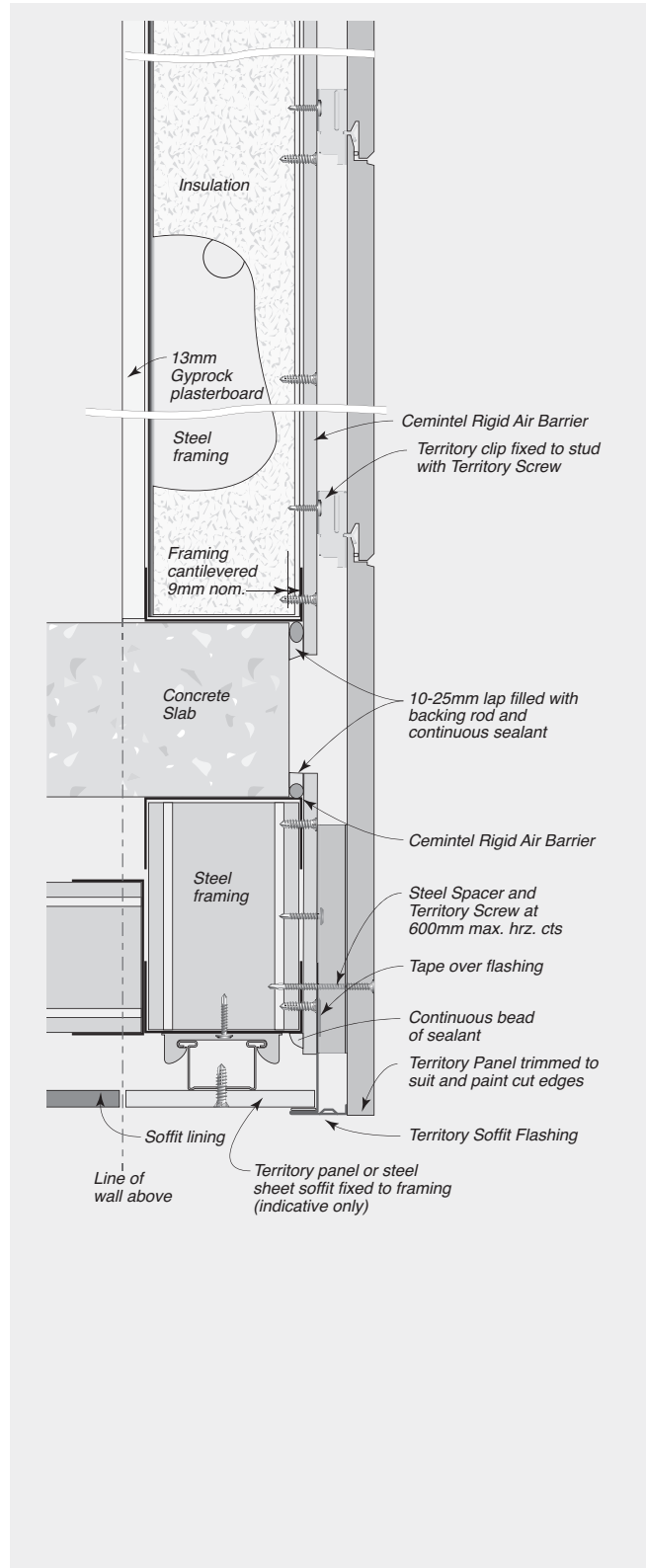
FIGURE 8.66 Composite Ceiling
