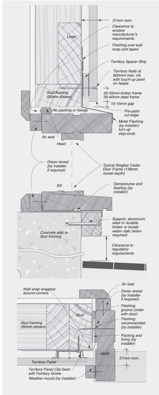
FIGURE 8.33 Typical Stegbar Sliding or Entry Door
