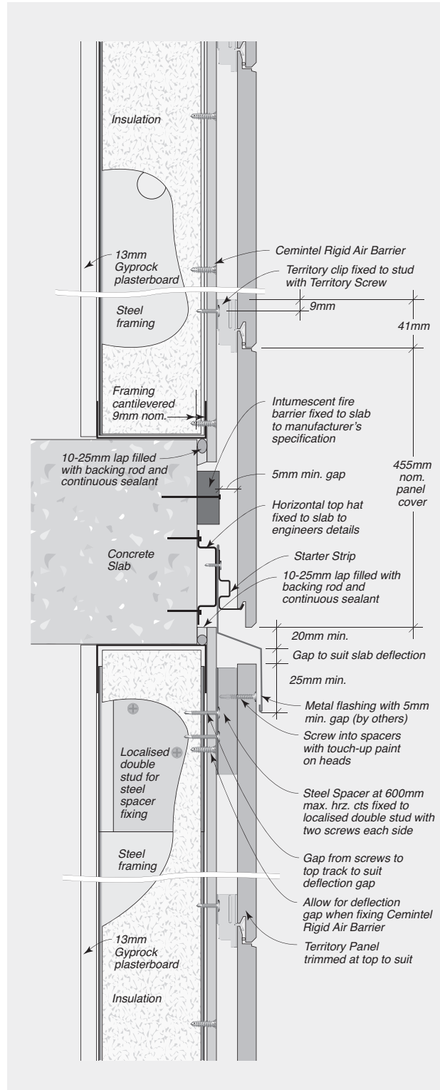
FIGURE 8.58 Edge Beam Detail
