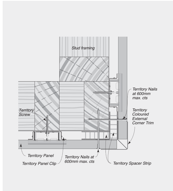
FIGURE 8.06 External Corner Detail – with Aluminium External Corner
