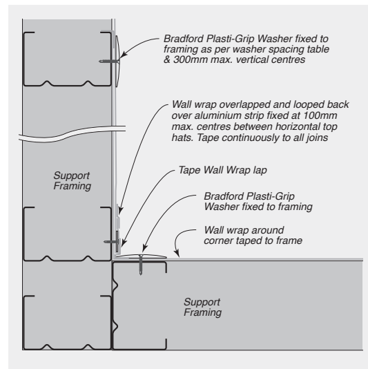
FIGURE 8.74 Internal Corner – Wall Wrap Overlapped
