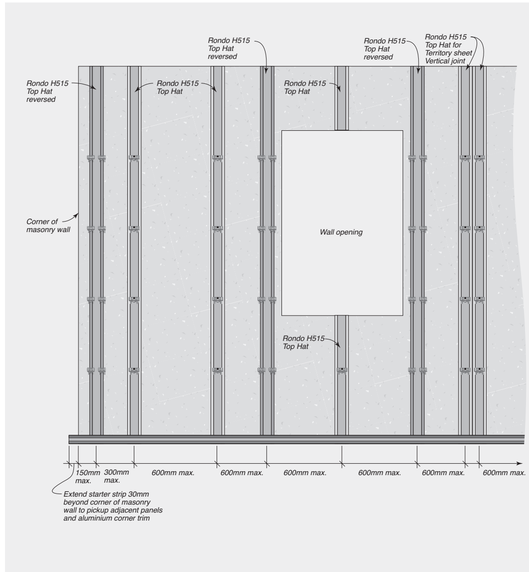
FIGURE 7.12 Masonry Overview Detail
