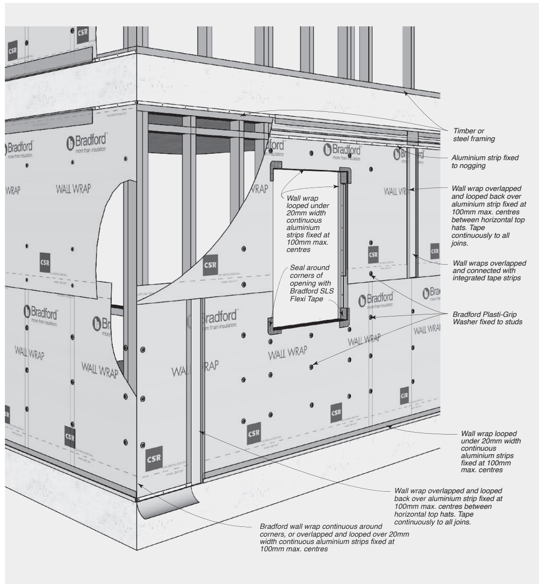
FIGURE 8.69 Typical Installation Overview – Soft Air Barrier
