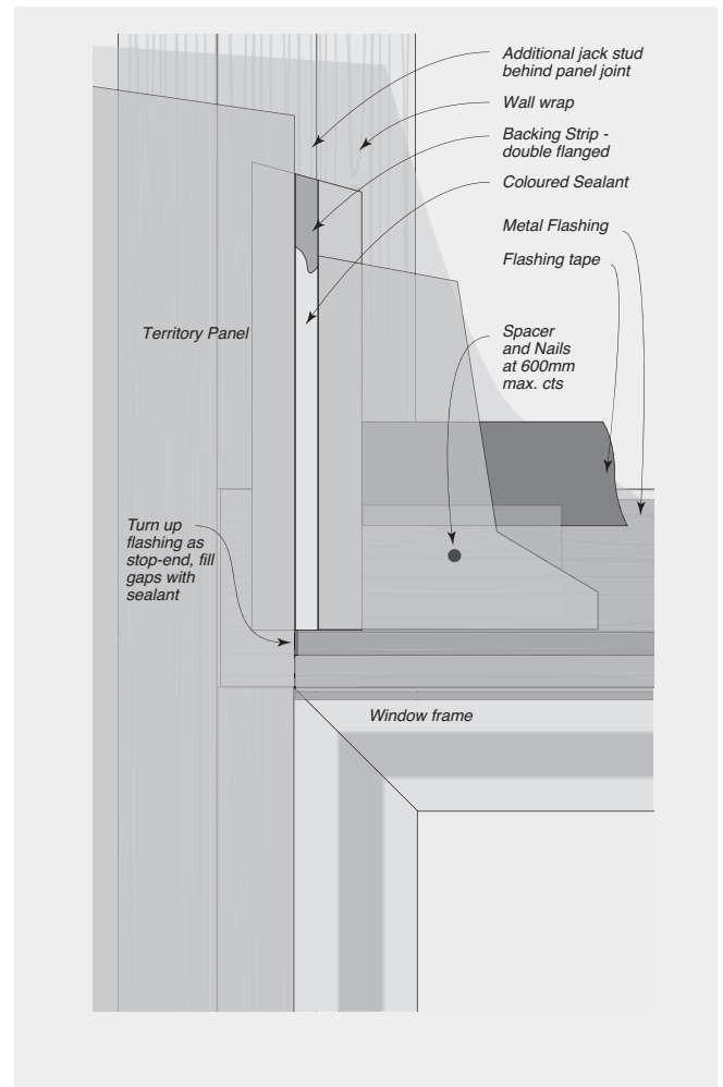
FIGURE 8.31 Typical Window
