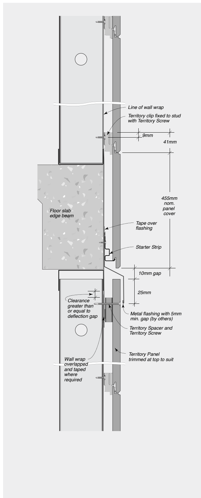
FIGURE 8.21 Edge Beam Detail – Horizontal Top Hat
