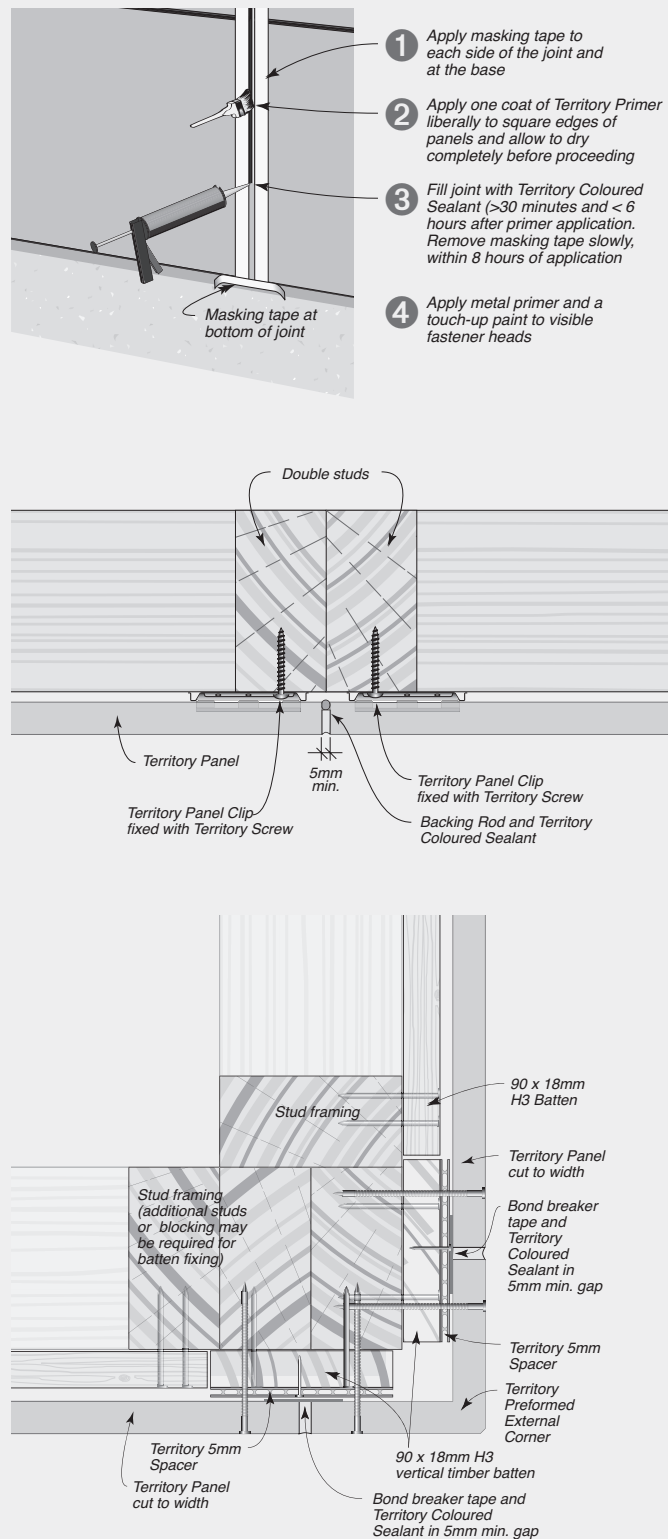
FIGURE 7.13 Typical Method for Sealing Vertical Joints
