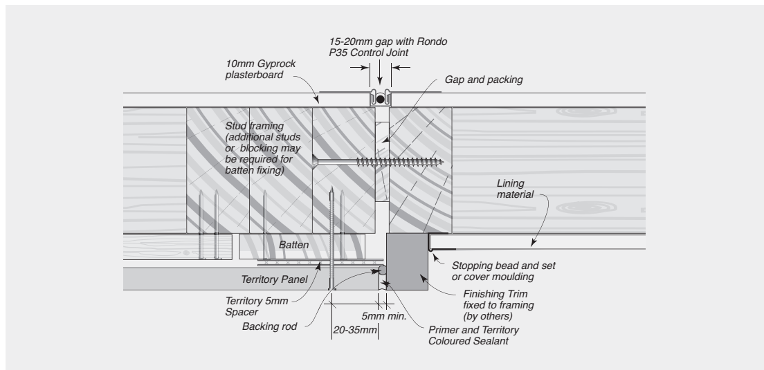
FIGURE 8.23 Typical Detail Junction with Fibre Cement Cladding System – Plan View
