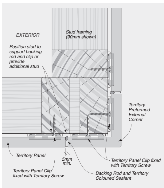
FIGURE 8.03 Performed External Corner – Plan View
