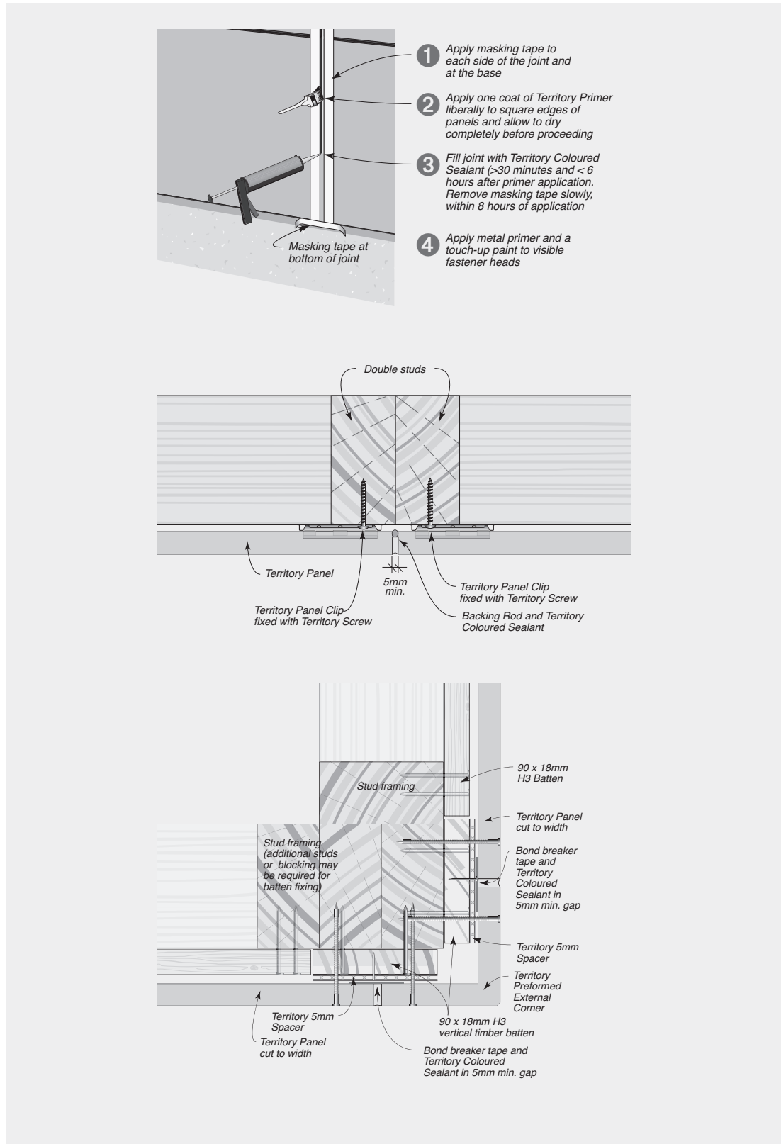
FIGURE 7.05 Typical Method for Sealing Vertical Joints
