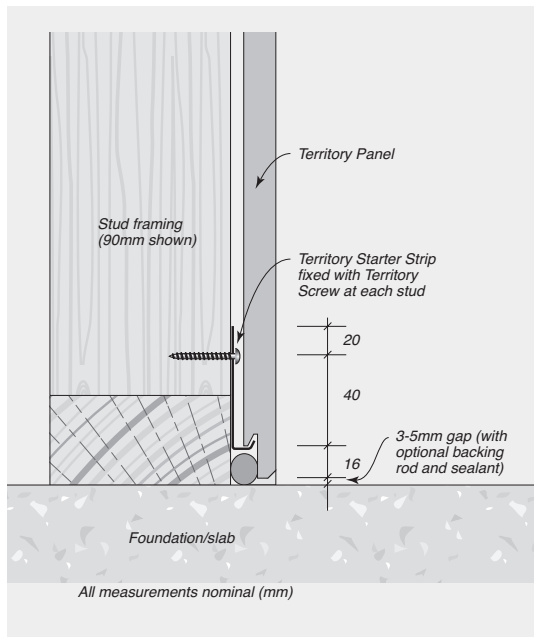
FIGURE 8.01 Base Detail – No Skirting
