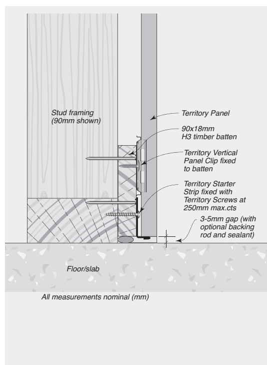
FIGURE 8.13 Base Details – With Sealant
