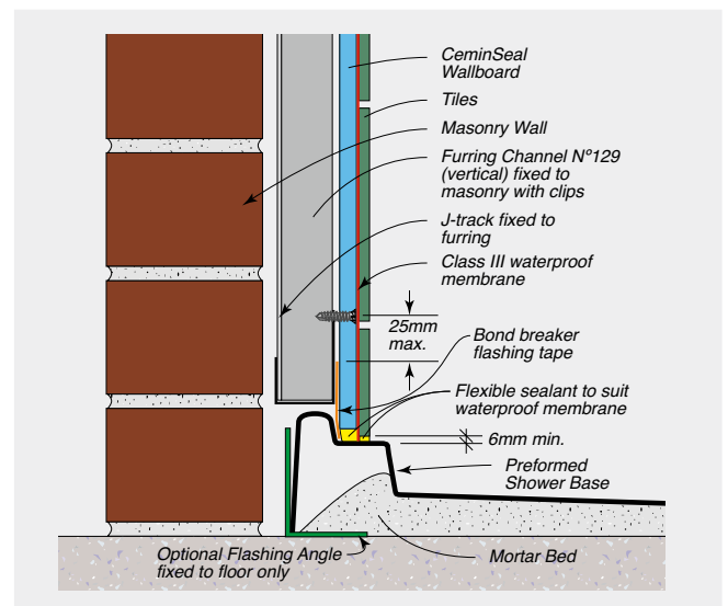
FIGURE 9.17 Preformed Shower Base
