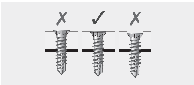
FIGURE 8.03 Fastener Driving
