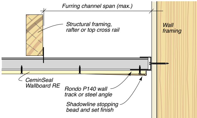
FIG 40: Perimeter Detail
