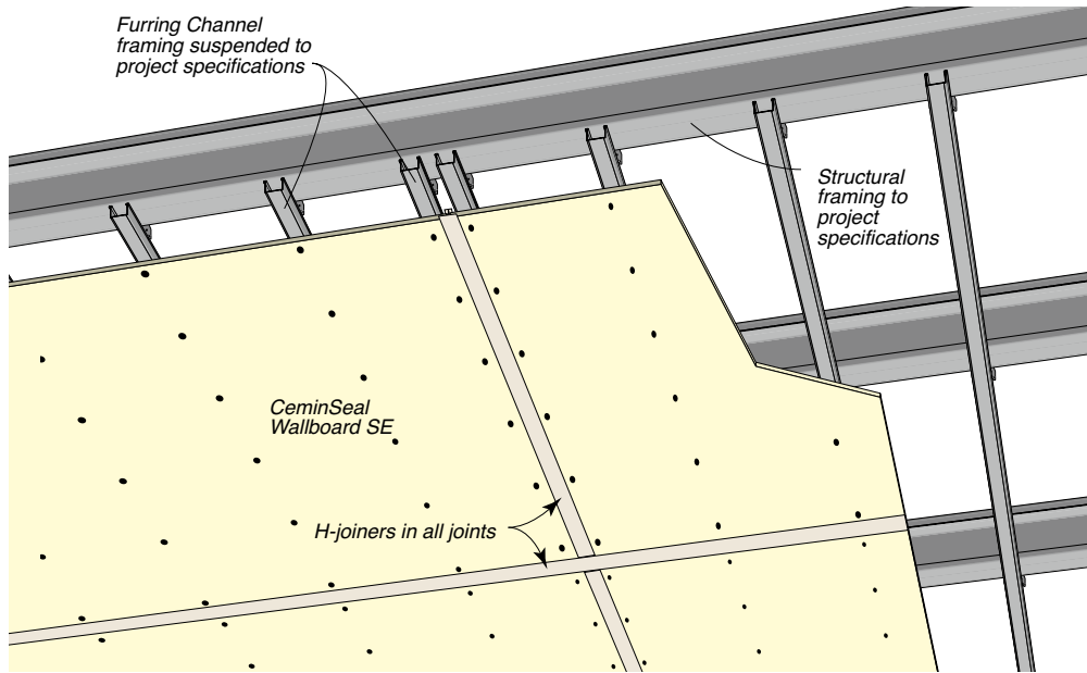
FIG 34: Sheet Module Control Joint – H-Mould Joint
