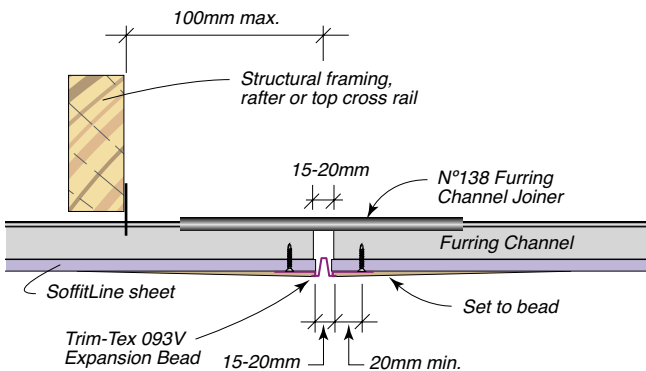
FIG 14: Framing & Sheet Module Control Joint
