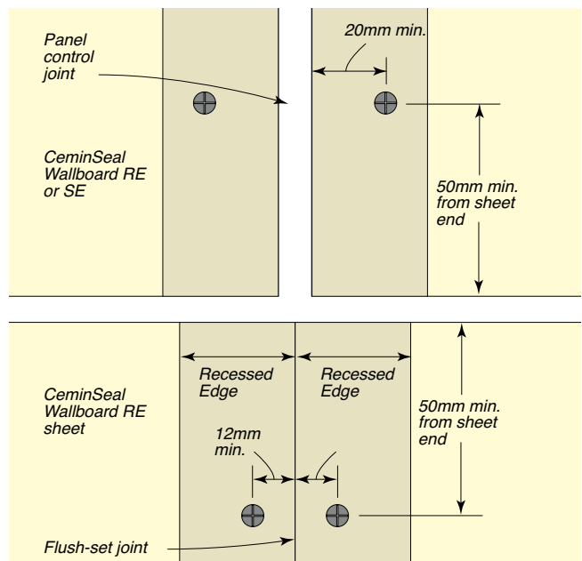
FIG 1: Fastener Positioning – Cemintel Wallboard
