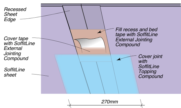
FIG 53: Flush-Set Jointing – External SoffitLine System Recessed Joint
