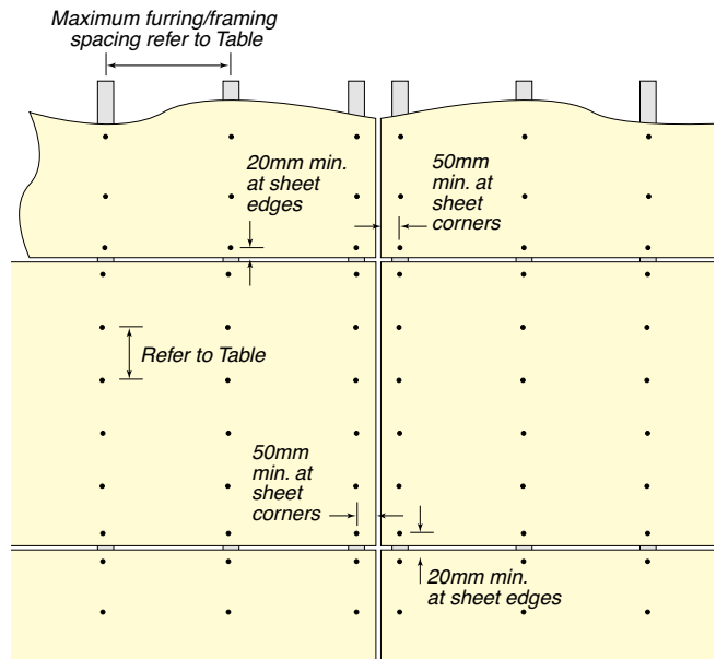
FIG 9: Fastener Fixing System for External Exposed Joint Ceiling Systems
