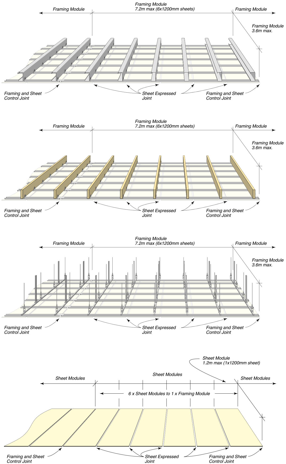
FIG 24: External Ceiling with Exposed Joints
