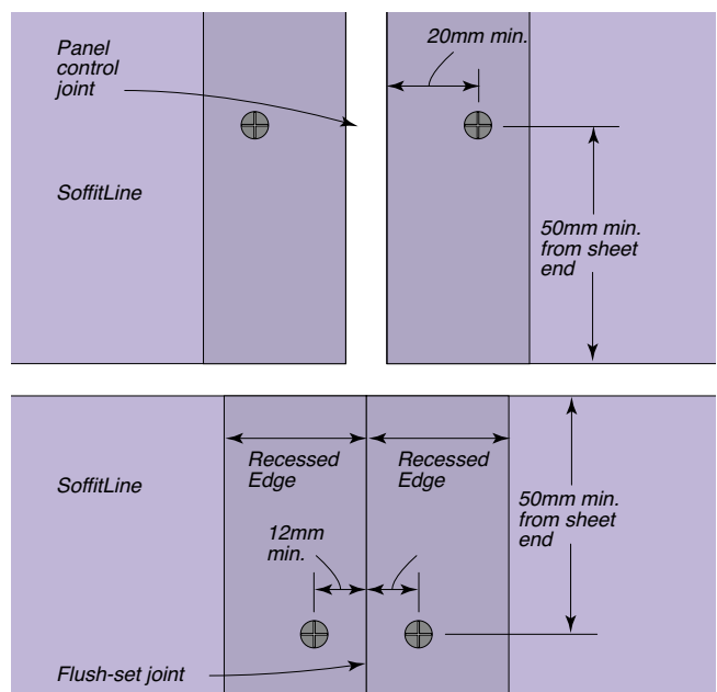
FIG 2: Fastener Positioning – Cemintel SoffitLine
