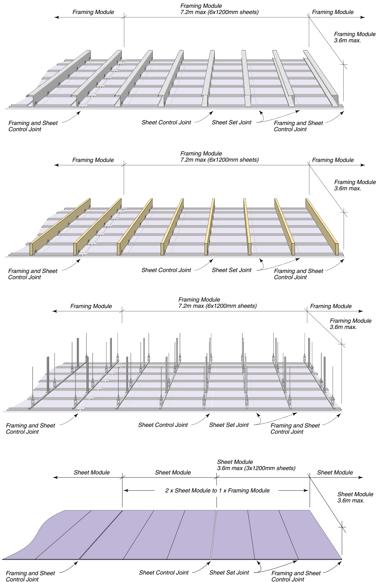
FIG 11: SoffitLine Ceiling System – External Ceiling with Flush-Set Joints
