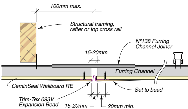
FIG 42: Framing & Sheet Module Control Joint
