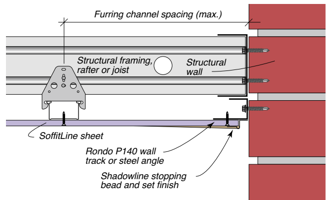
FIG 16: Perimeter Detail
