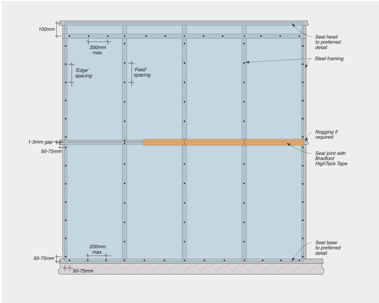
FIGURE 6.04 SHEET FIXING - HORIZONTAL SHEETING* - STEEL FRAMING. NON-LOADBEARING FRAMING SHOWN.
