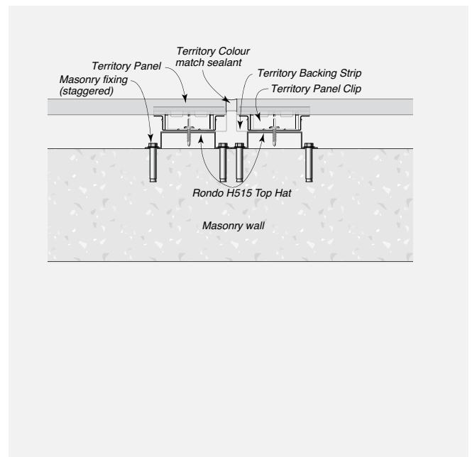
FIGURE 8.48 Vertical Panel Joint (Option 2)
