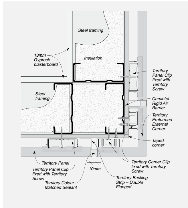
FIGURE 8.54 External Corner Detail – with Preformed Corner
