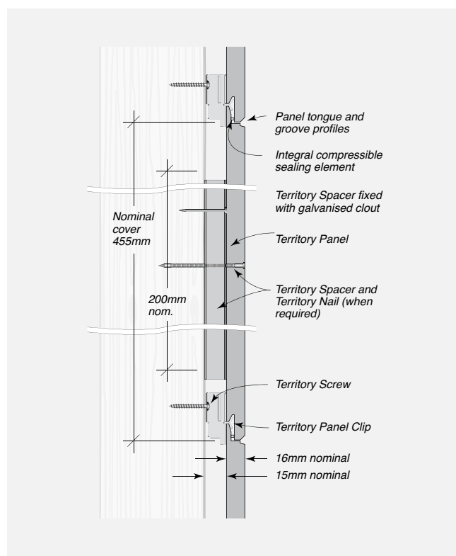
FIGURE 7.04 Typical Territory System Cross Section for Timber Framing for when face fixing is required – Elevation
