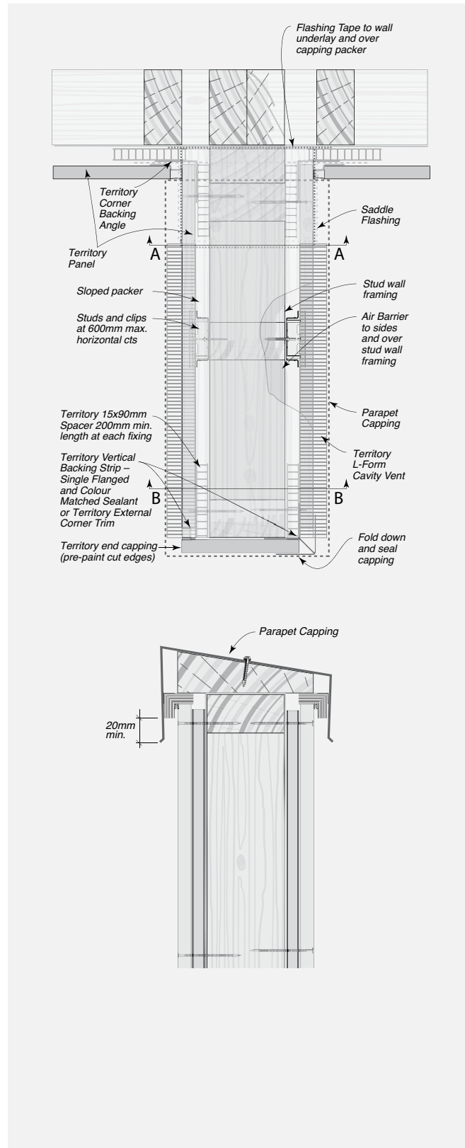
FIGURE 8.35 Parapet Wall
