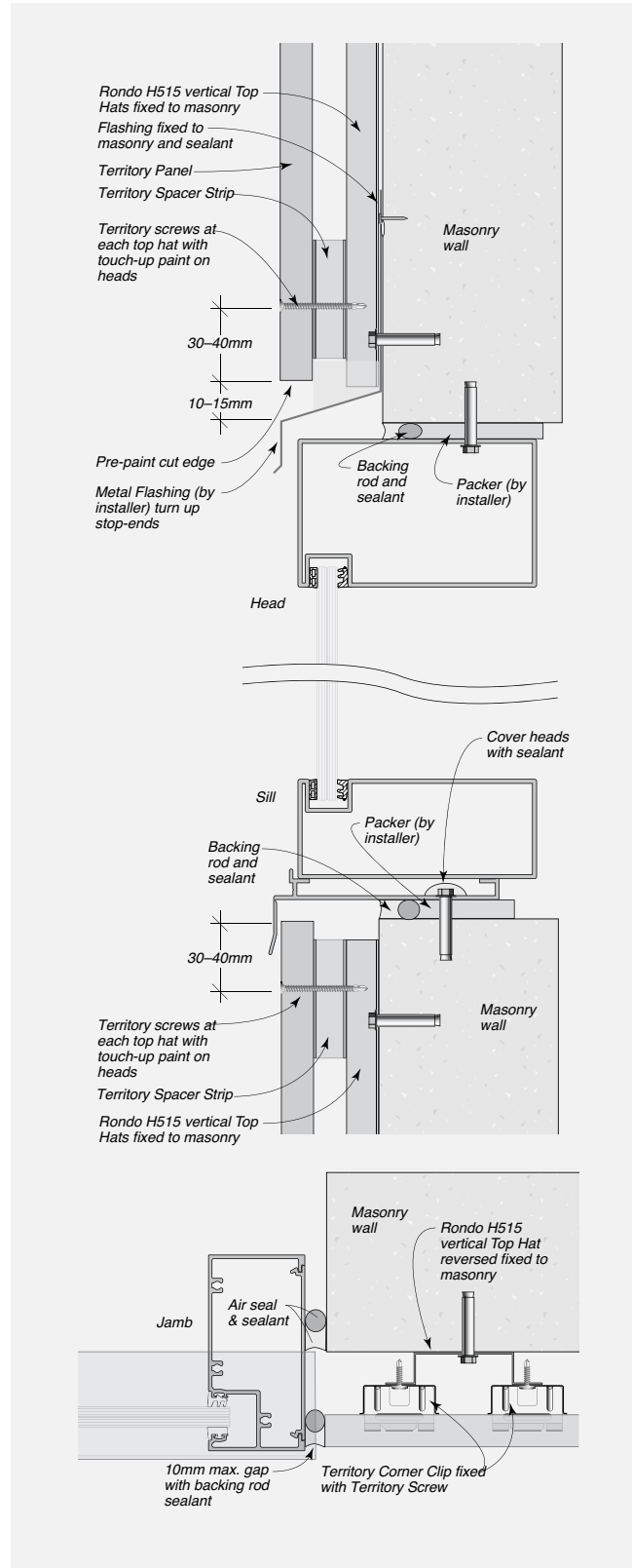
FIGURE 8.50 Generic Commercial Window for Masonry Substrates
