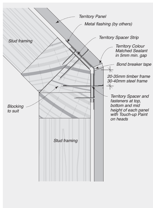
FIGURE 8.06 Obtuse Angle Corner with Metal Flashing and Colour Matched Sealant – Plan View
