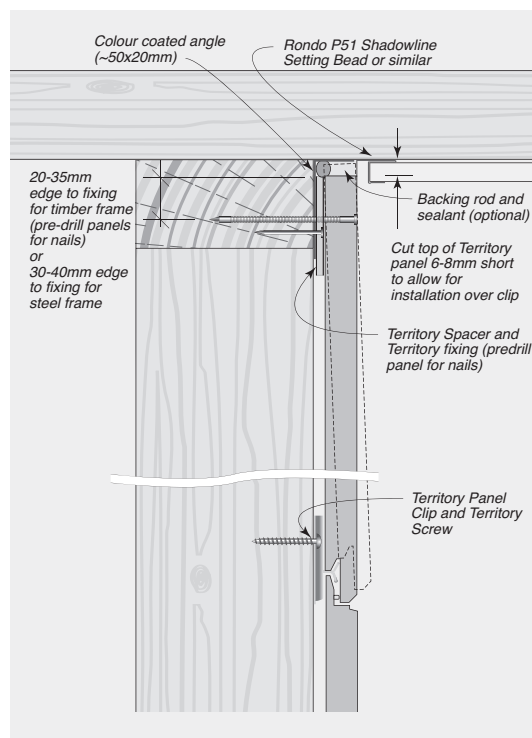
FIGURE 8.08 Head Detail – With Shadowline Trim
