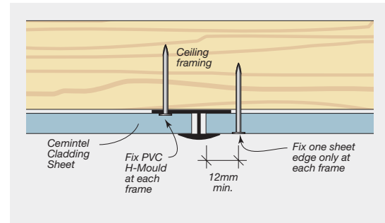
FIGURE 6.16 Edge Joint with PVC H-Mould – Ceiling
