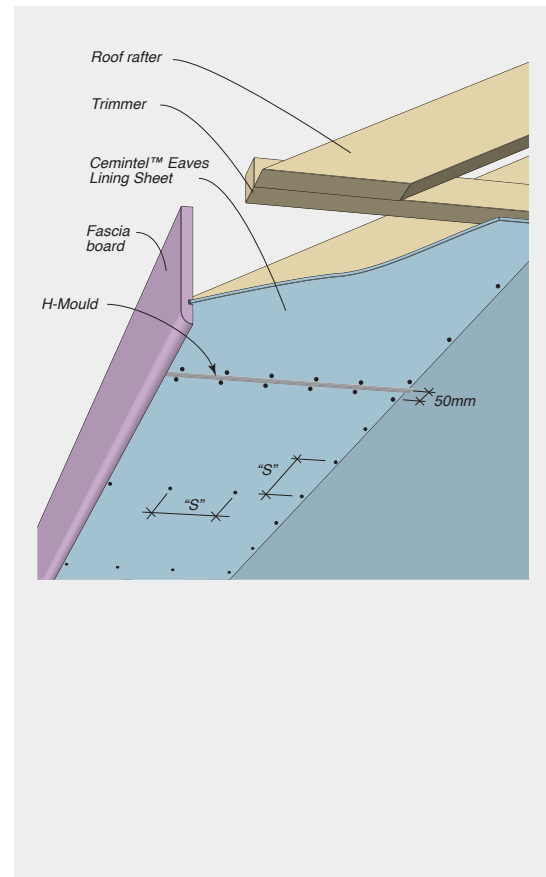
FIGURE 6.17 Typical Eaves Fixing Layout
