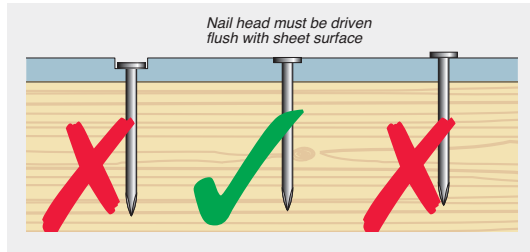
FIGURE 6.03 Fastener Driving
