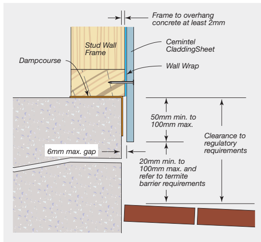
FIGURE 6.04 Base Detail
