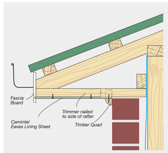
FIGURE 6.12 Typical Installation Detail for Eaves
