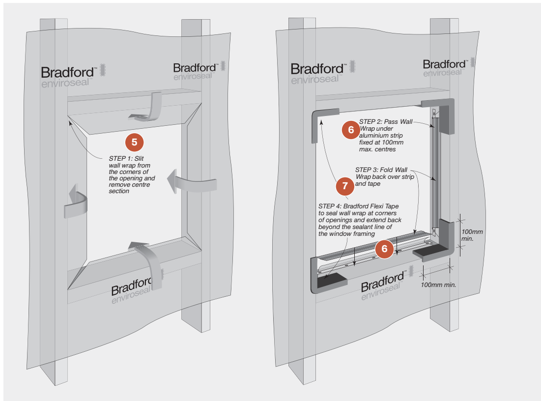
FIGURE 7.18 Treatment at Window/Door Openings - Soft Air Barrier
