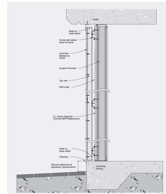
FIGURE 6.11 Typical Barestone External Fire Rated Installation. Pressure Equalised Ventilated Cavity System
