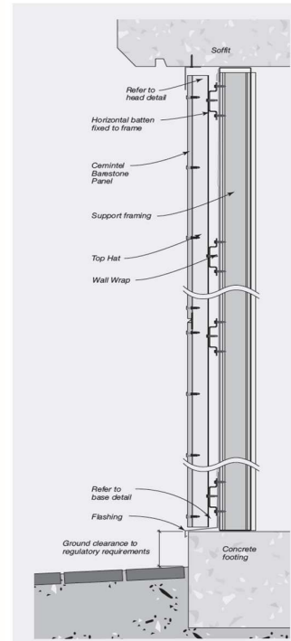
Typical Barestone External Wall System Cross Section for Steel Framing
