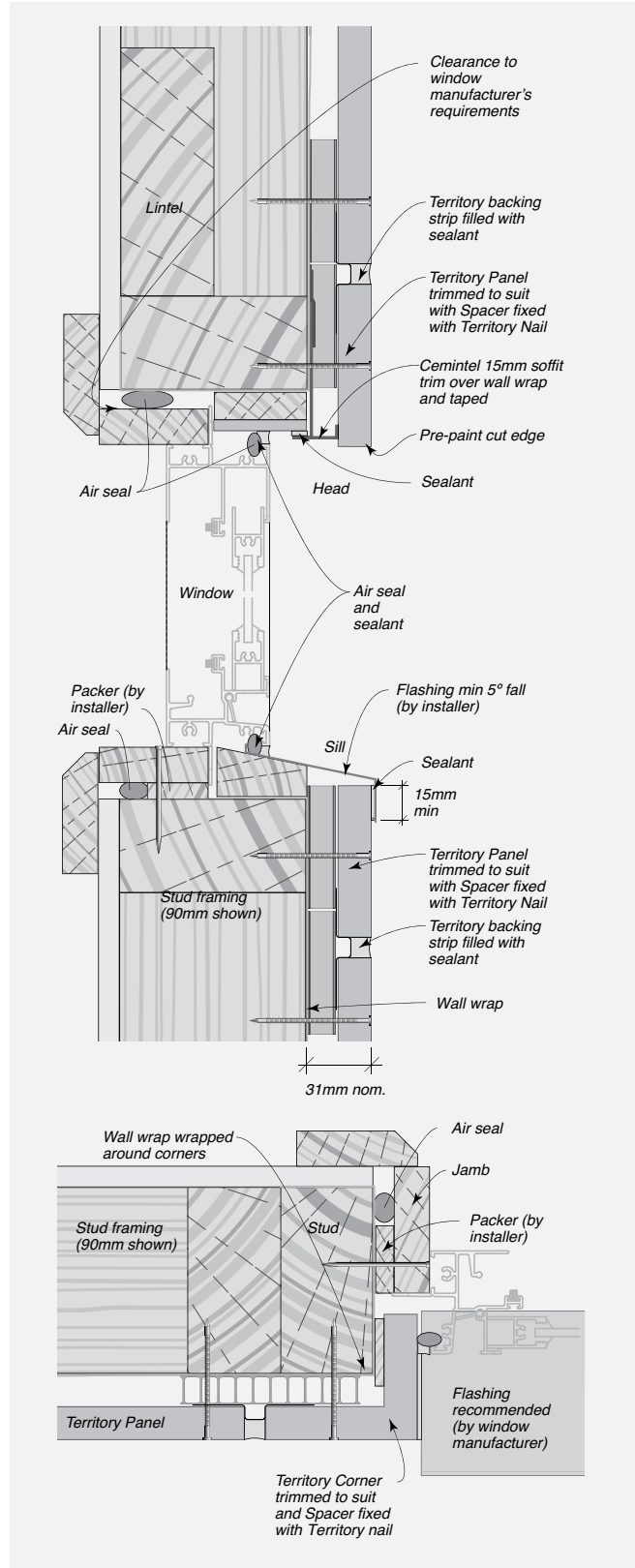
FIGURE 8.28 Window Reveal
