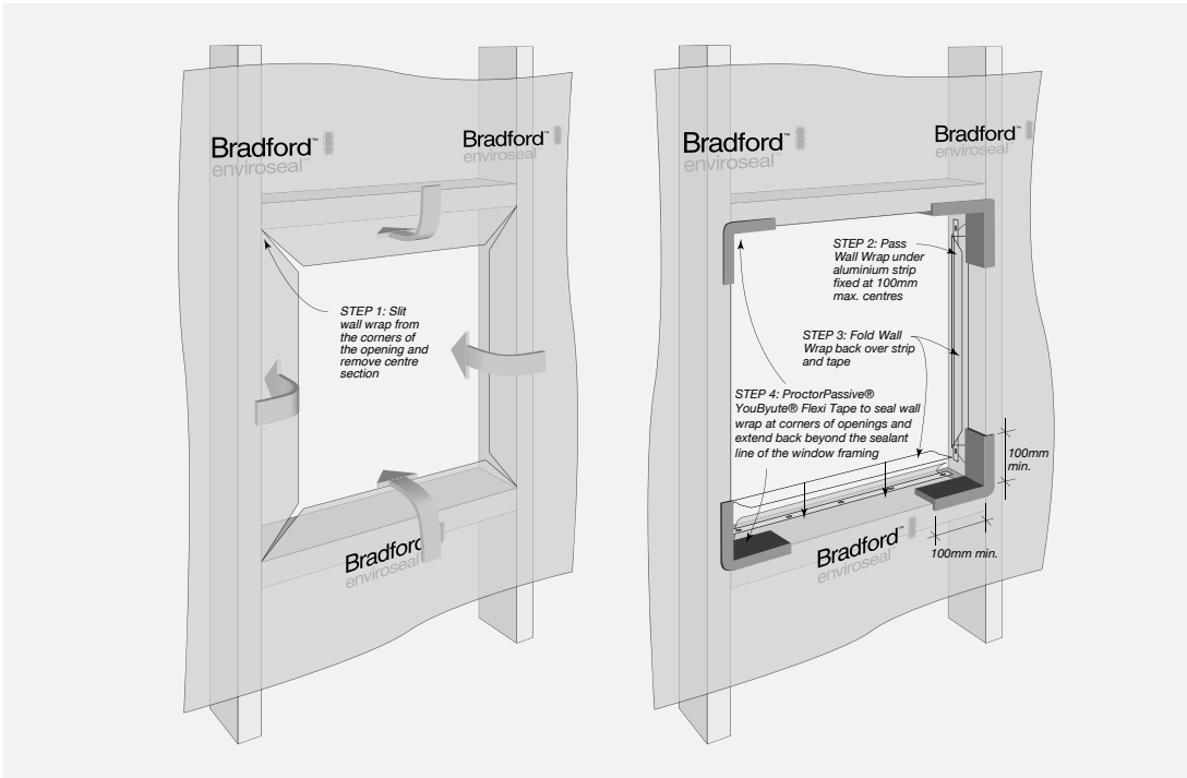
FIGURE 8.78 Wall Wrap Installation at Window/Door Opening
