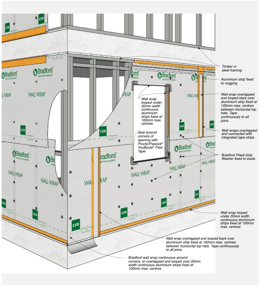
FIGURE 8.65 Typical Installation Overview – Soft Air Barrier
