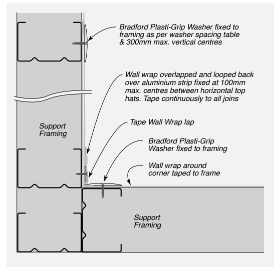
FIGURE 8.70 Internal Corner – Wall Wrap Overlapped
