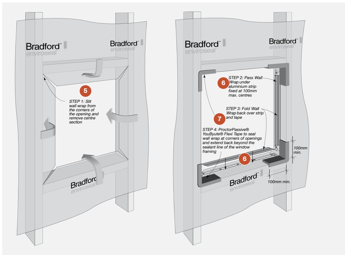
FIGURE 7.18 Treatment at Window/Door Openings - Soft Air Barrier
