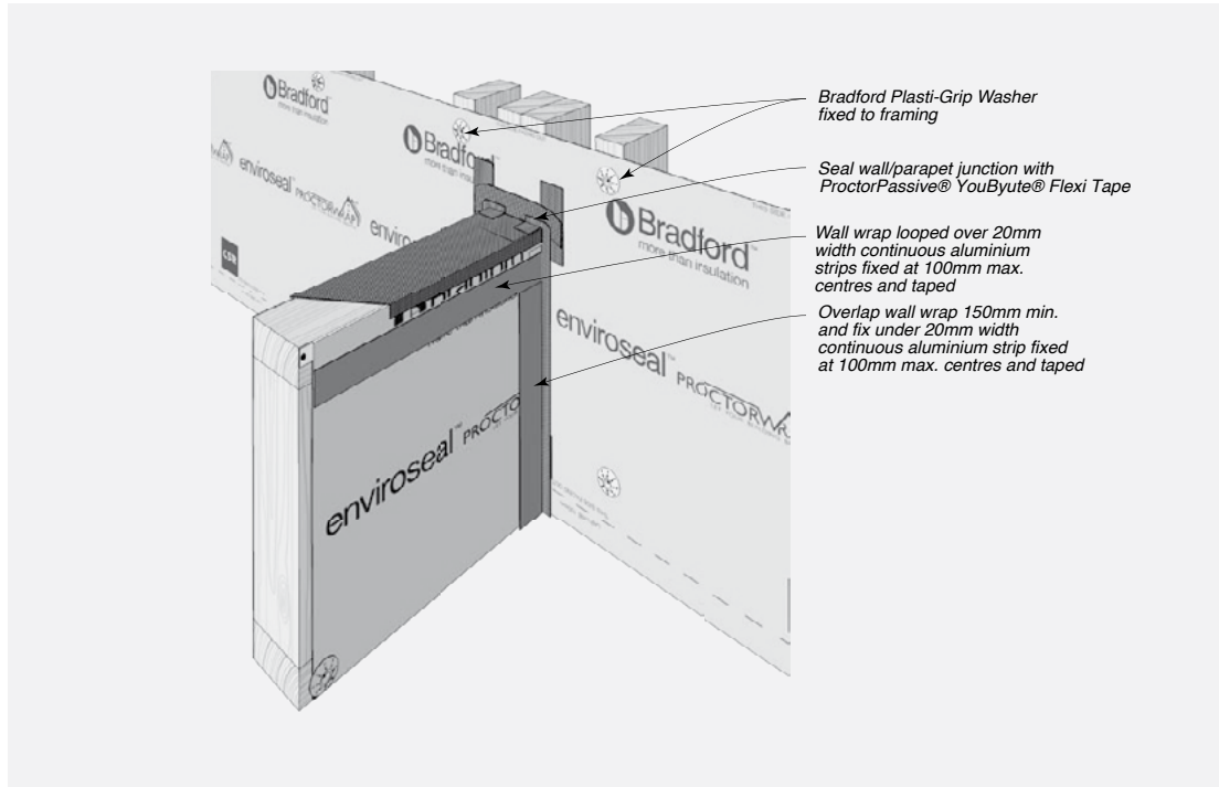
FIGURE 8.79 Wall Wrap Installation at Parapet Junction – Timber or Steel Framing
