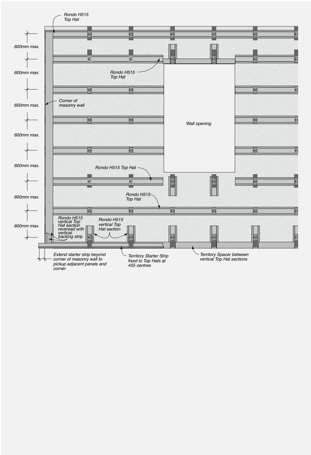
FIGURE 7.14 Masonry Overview – Detail
