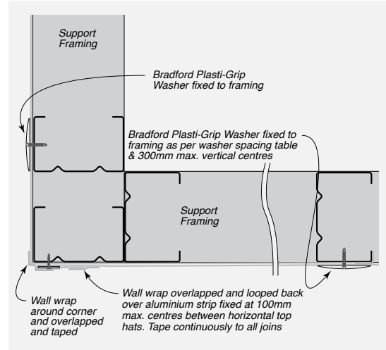
FIGURE 8.67 External Corner – Wall Wrap Overlapped
