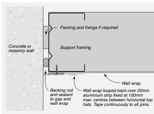
FIGURE 8.69 Abutment to Concrete or Masonry Wall
