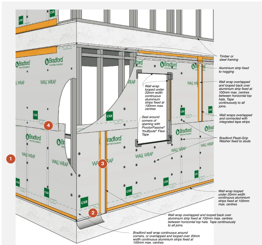
FIGURE 7.17 Typical Soft Air Barrier Installation
