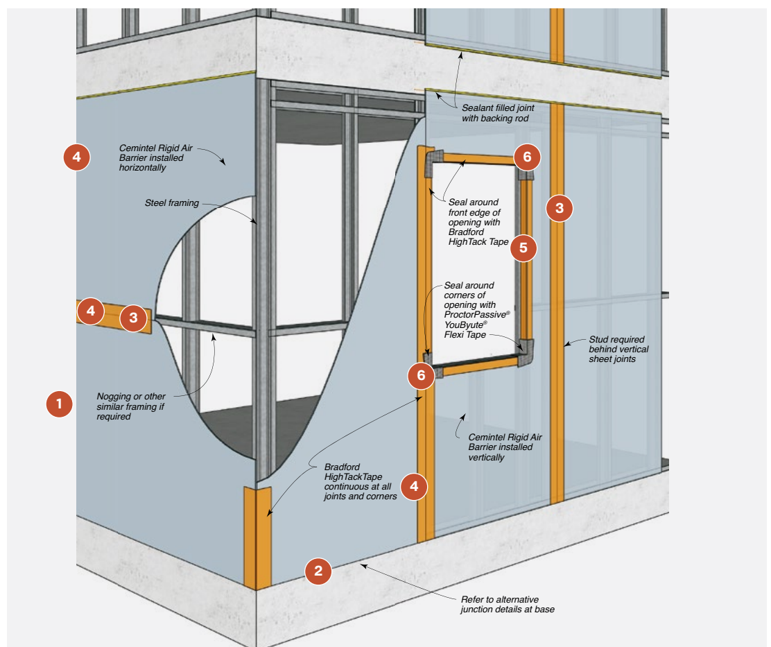
FIGURE 7.15 Typical Rigid Air Barrier Installation
