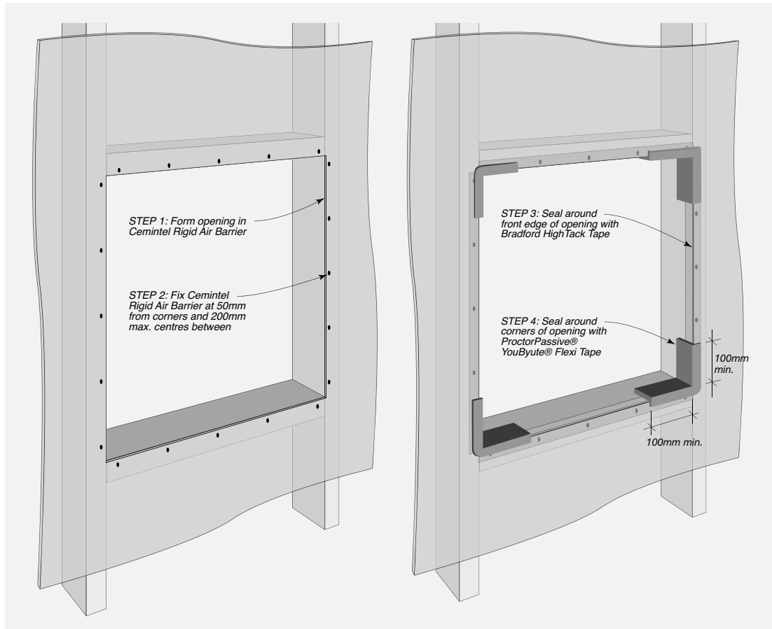
FIGURE 7.16 Treatment at Window/Door Openings – Rigid Air Barrier
